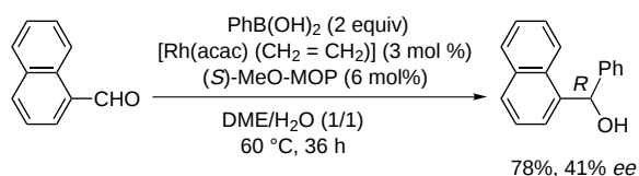
Scheme 2. Asymmetric addition.
